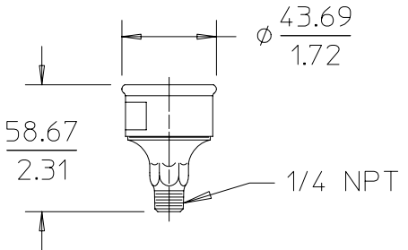
MUFFLER ASM. (SHIPPED UNATTACHED)
